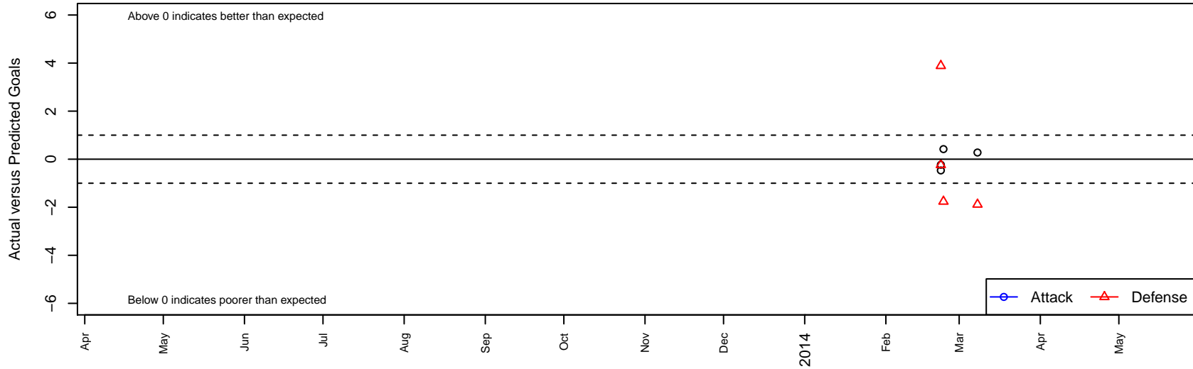
Claremont Star SC B00 Dots are actual minus expected GF (blue circles) and GA (red triangles). Blue line is smoothed change in attack strength. Red is smoothed change in defense strength.
